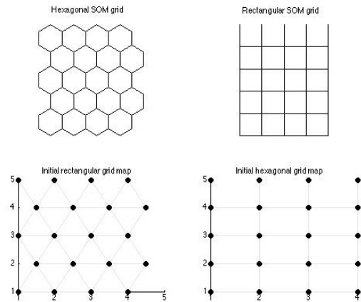
Figure 4: Initial grid example (hexagonal & rectangular).
